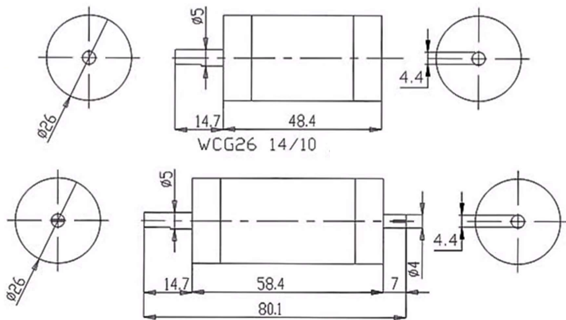
Rotary Solenoid Without Limit
