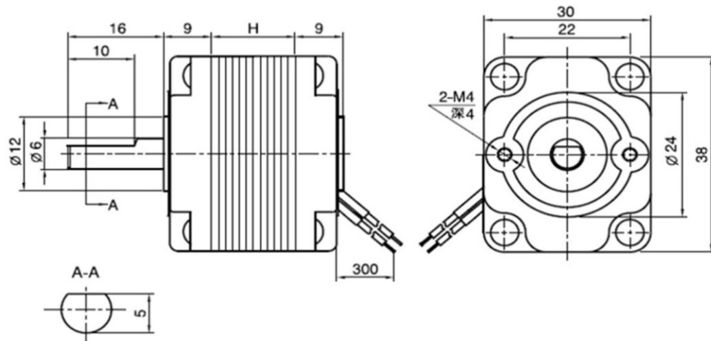
Rotary Solenoid Without Limit
