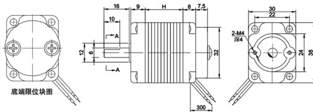
Rotary Solenoid With Limit
