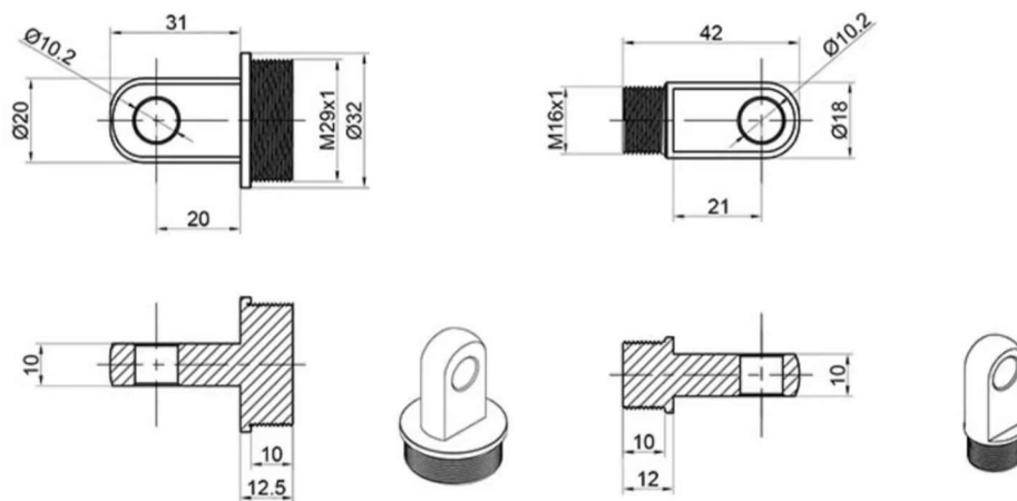
Connector ①:
